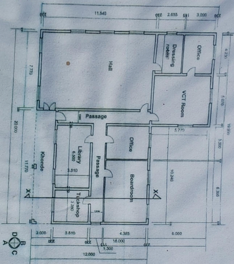
FLOOR PLAN scale 1:100
